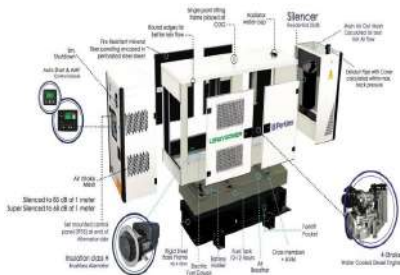
ATP ENCLOSURE/CANOPY
